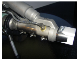
Separate heating and control of extrudate and pre-heating air
